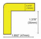
Corner Guard Type H
