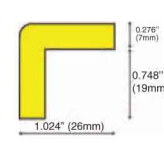
Corner Guard Type E
